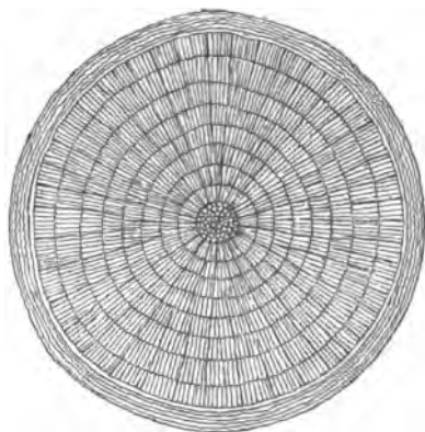
FIG. 1.—Section of an Eight-year-old Oak tree.
